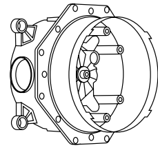
iBox® universal Basic set iBox universal # 01800180 Extension set 25 mm for too deep installation: # 13595000 Extension set 22 mm for too low installation depths: # 13596000 for escutcheons of diameter 170 mm # 13597000 for escutcheons of diameter 150 mm # 97407000 for escutcheons of diameter 172 mm # 15597000 for PuraVida
