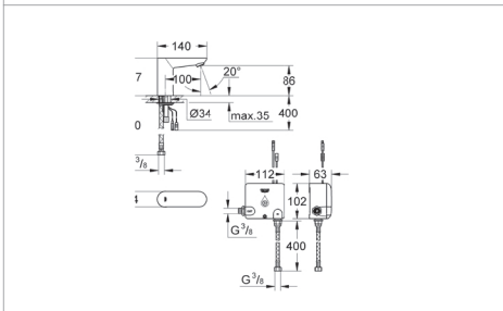
36 384 000 Powerbox with Euroeco Cosmopolitan E Powerbox with internal energy storage without mixing device CE approved
