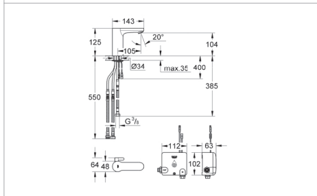
36 386 000 Powerbox with Eurosmart Cosmopolitan E Powerbox with internal energy storage with mixing device CE approved
