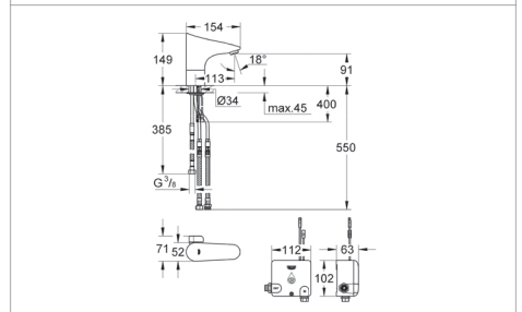
36 387 000 Powerbox with Europlus E Powerbox with internal energy storage with mixing device CE approved
