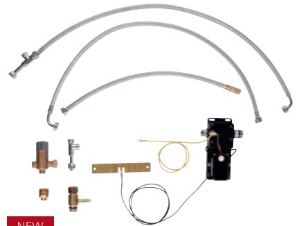
30 309 000 Retro-Fit set for upgrading any GROHE pull-out kitchen tap with FootControl technology
