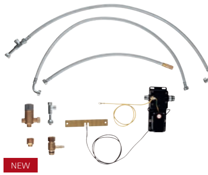
30 309 000 Retro-Fit set for upgrading any GROHE pull-out kitchen tap with FootControl technology
