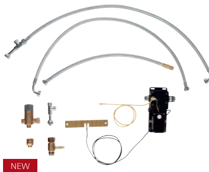
● 30 309 000 Retro-Fit set for upgrading any GROHE pull-out kitchen tap with FootControl technology
