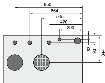
MGK-2-130
