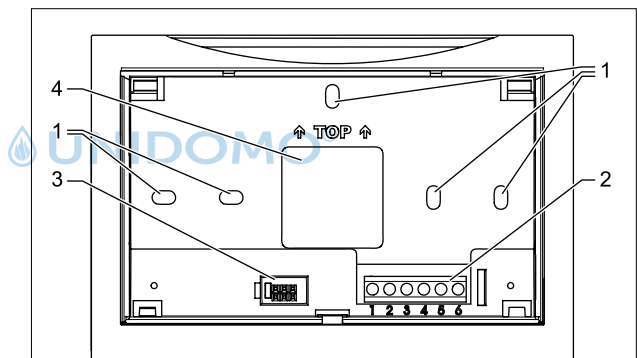
Abb. 4.5 Montage Wandsockel
