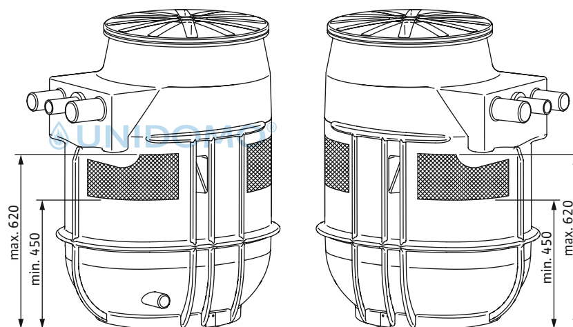
Fig. 7: Inlet areas
