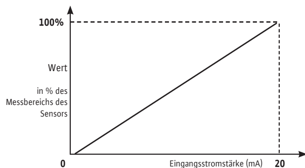
Sensorsignal 0–20 mA
