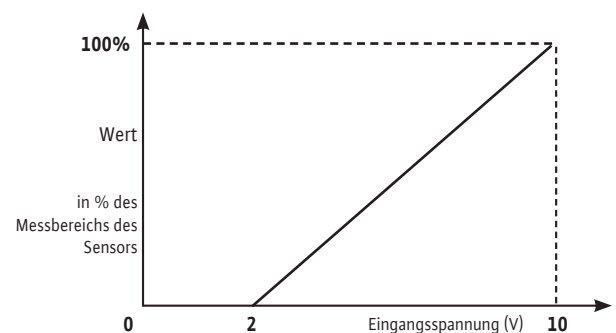
Sensorsignal 2–10 mA
