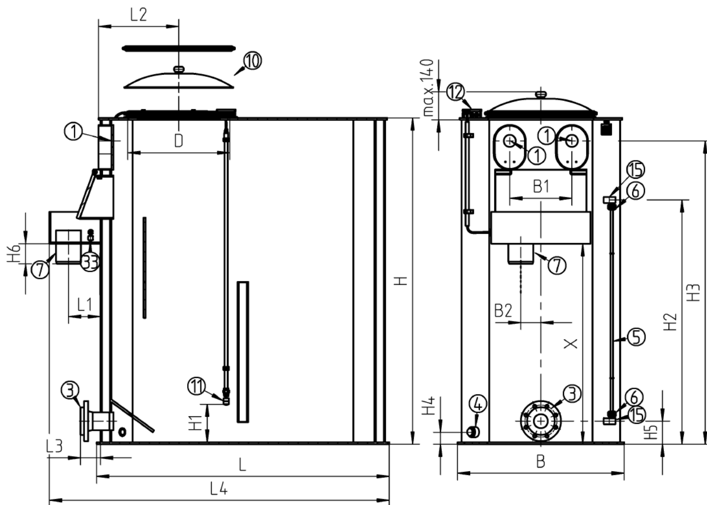
VBH 800-1000L-angular-FLA
