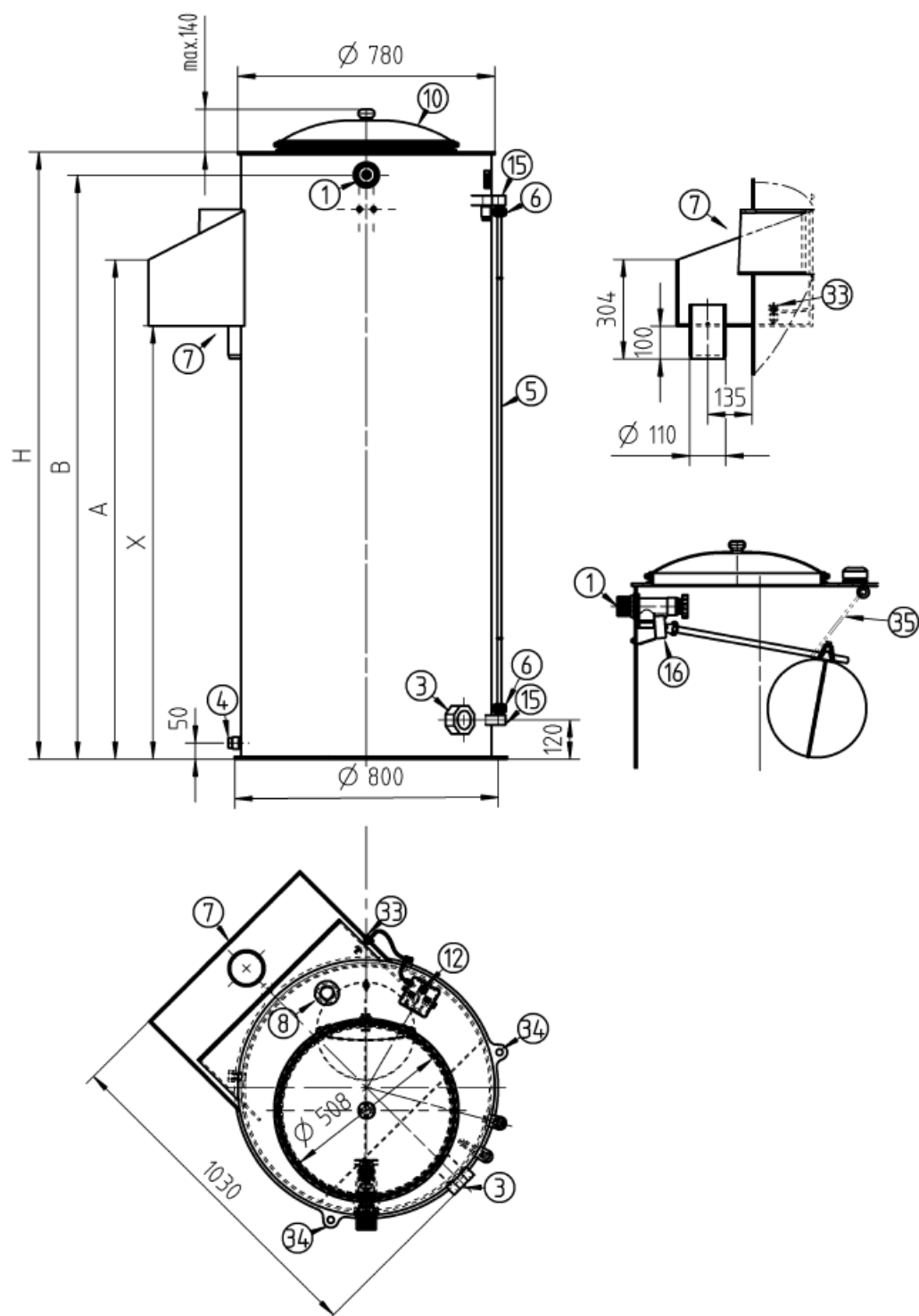
Fig. 1g: Dimensional drawing of break tank 540L-round-ACS
