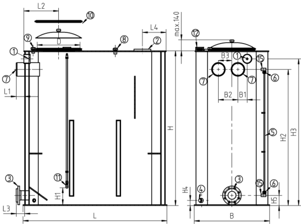
VBH 1500-3000L-angular-GIII
