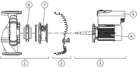
Fig. 3: Functional assemblies
