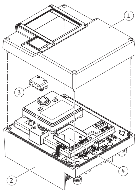
Fig. 25: Electronic module
