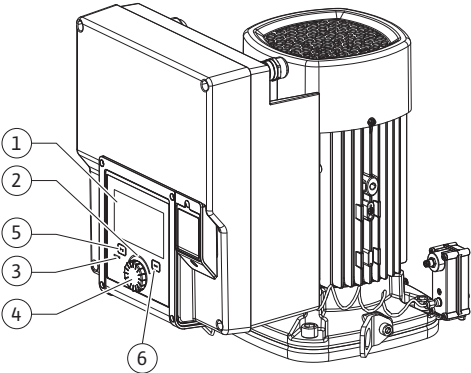
Fig. 28: Operating elements
