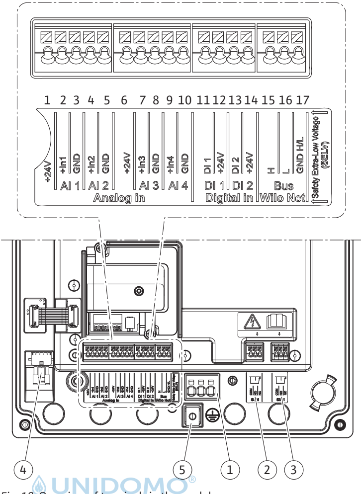
Fig. 19: Overview of terminals in the module
