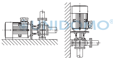
Fig. 7: Atmos GIGA-B
