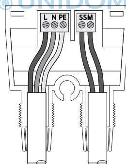
Fig. 22: Raccordement
