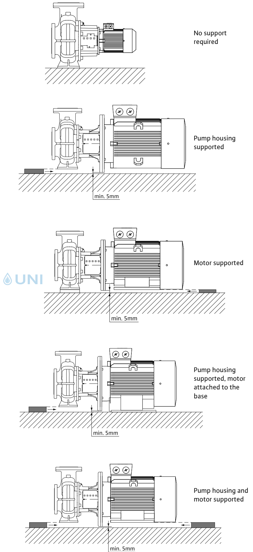
Fig. 14: Installation examples BL
