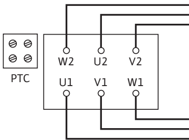
Fig. 46: Δ-schakeling
