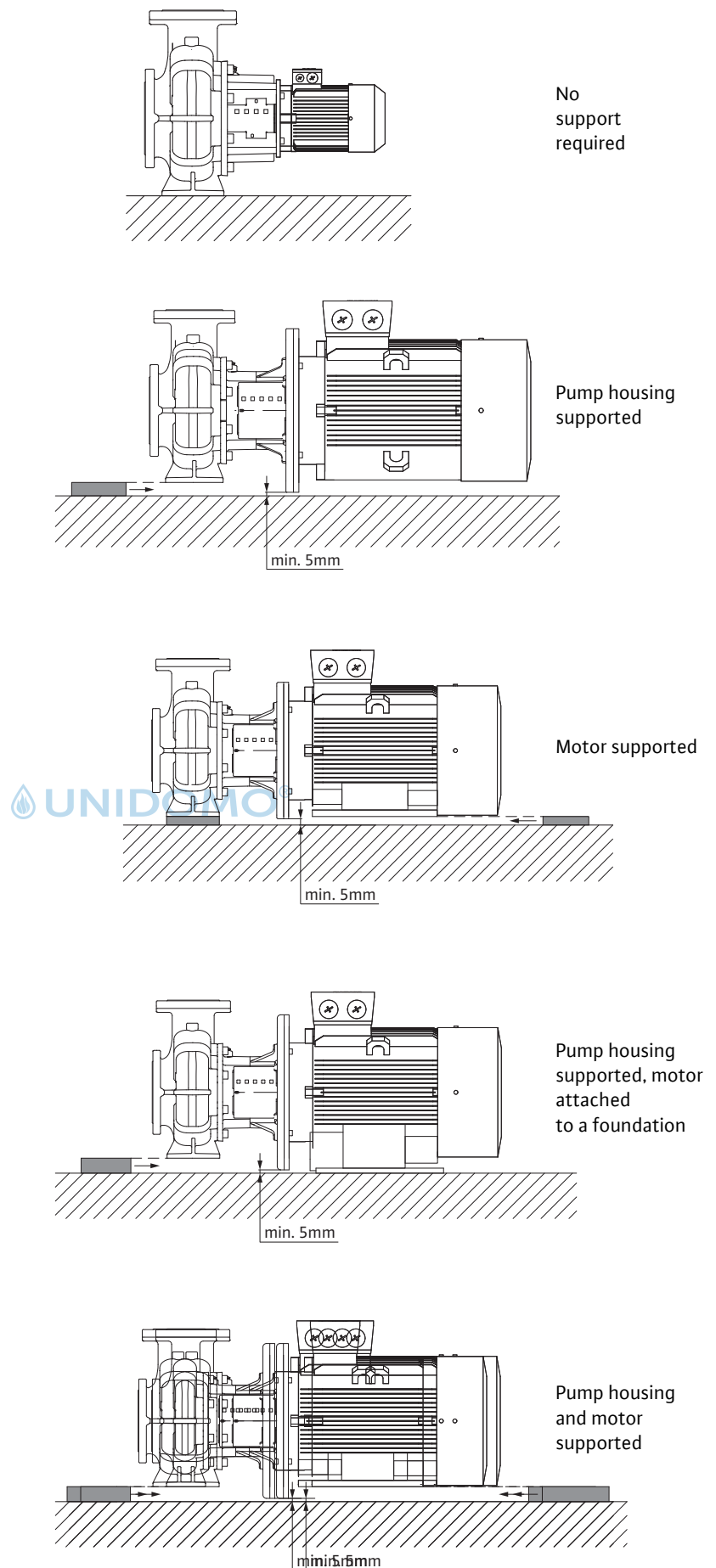
Fig. 42: Installation examples BL
