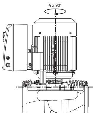
Fig. 19: Permitted installation positions with vertical motor shaft
