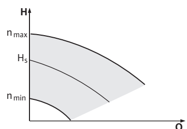
Fig. 41: Manual control mode
