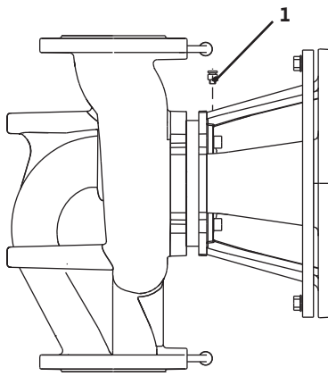
Fig. 38: Ventilation valve
