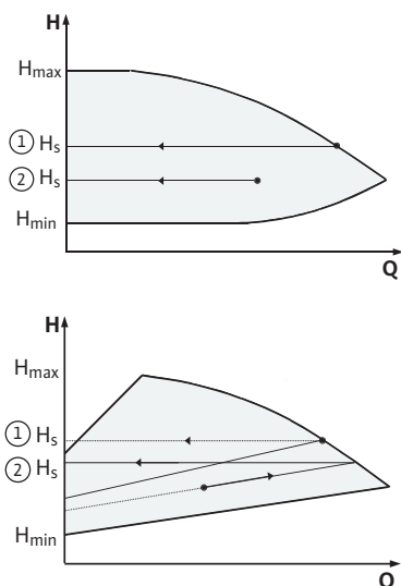
Afb. 40: Regeling \Delta p\text{-}c/\Delta p\text{-}v
