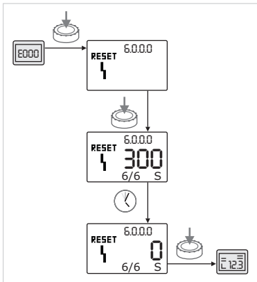
Fig. 48: Acknowledging error type B (X = Y)
