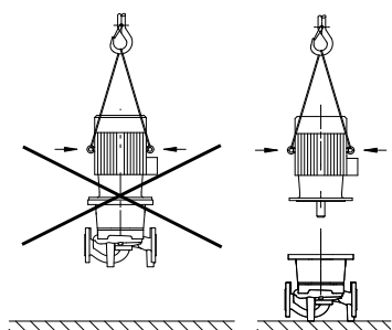
Fig. 8: Transporting the motor
