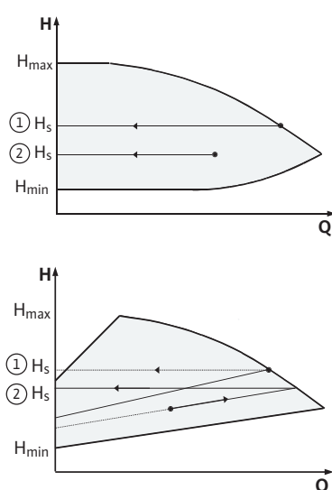
Fig. 40: \Delta p -c/ \Delta p -v control
