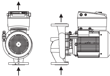
Fig. 17: Arrangement of the components upon delivery
