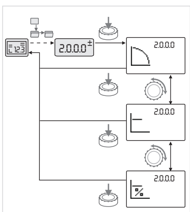
Fig. 36: Setting with return to the status page
