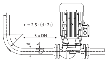
Fig. 9: Settling section before and after the pump
