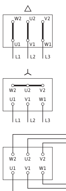
Fig. 11: Mains connection
