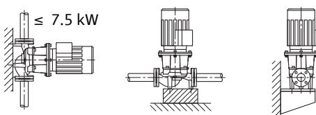
Fig. 6: View of IPL – Installation on a base
