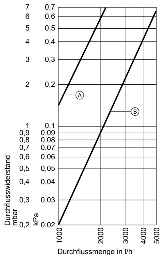
Vitocell 100-E
