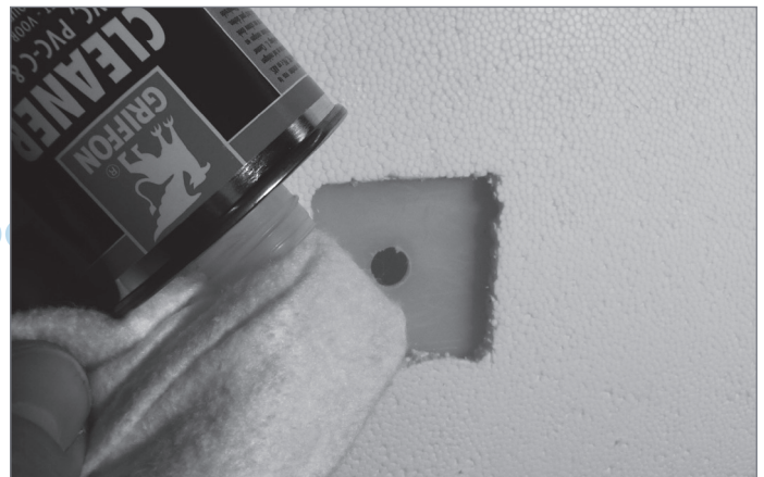
4. Clean both glue areas with acetone or provided cleaner
