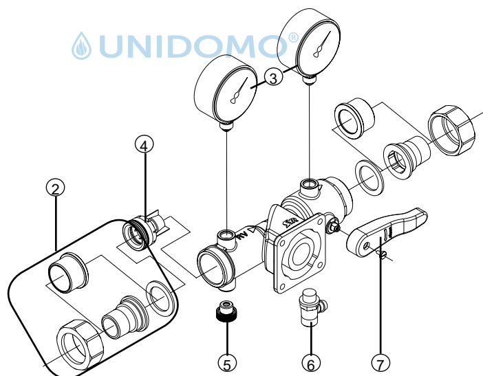
HWS- Flansch 2000
