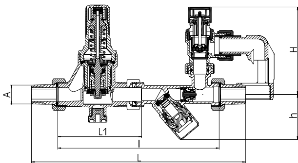
DN 15
