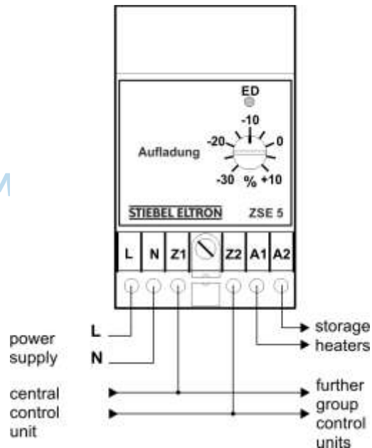
Connection diagram ZSE 5
