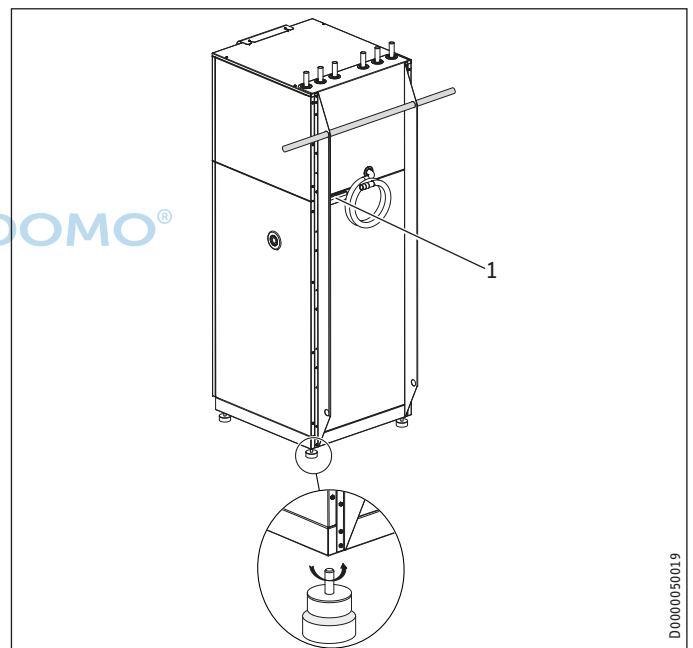
1 Cable entry
