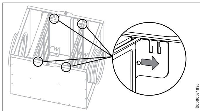
2 Filter frame
