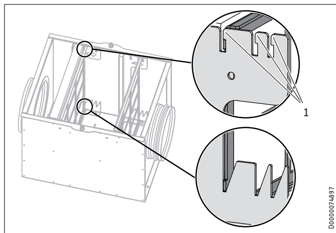
1 Locking tab
