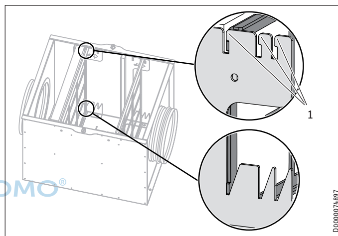
1 Locking tab
