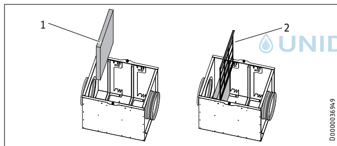
1 Filter
