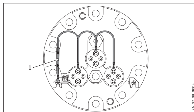
1 Corrosion resistor 390 Ω
