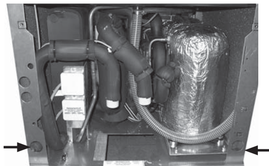
AuraModul 12-17 kW
