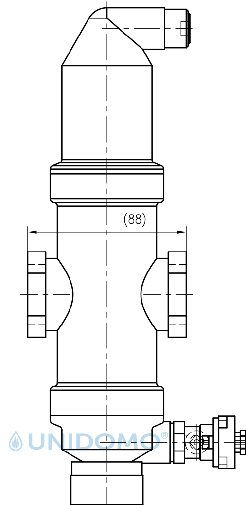
Front view
