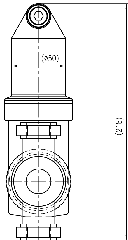
Side view
