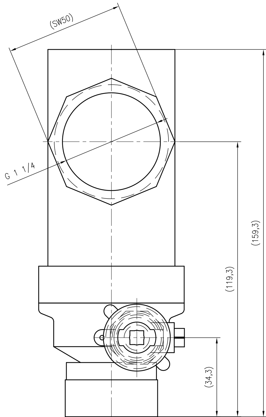
Side view
