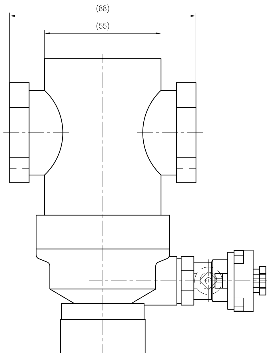
Front view
