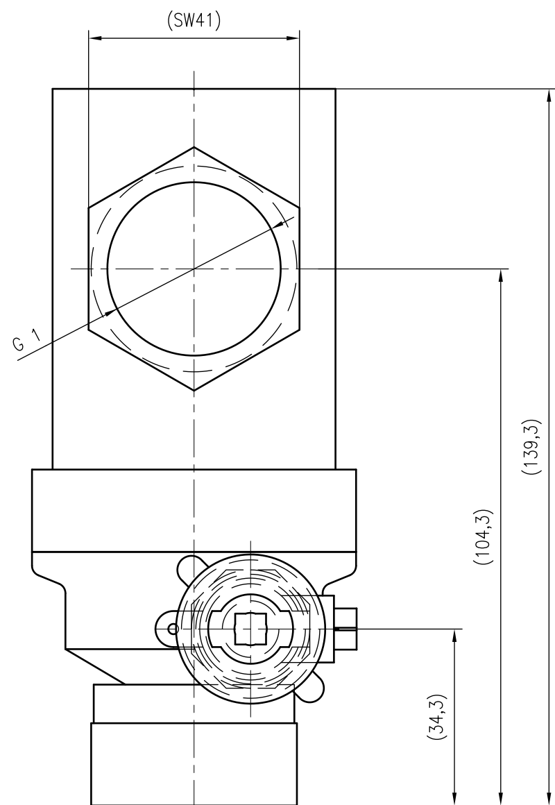
Side view
