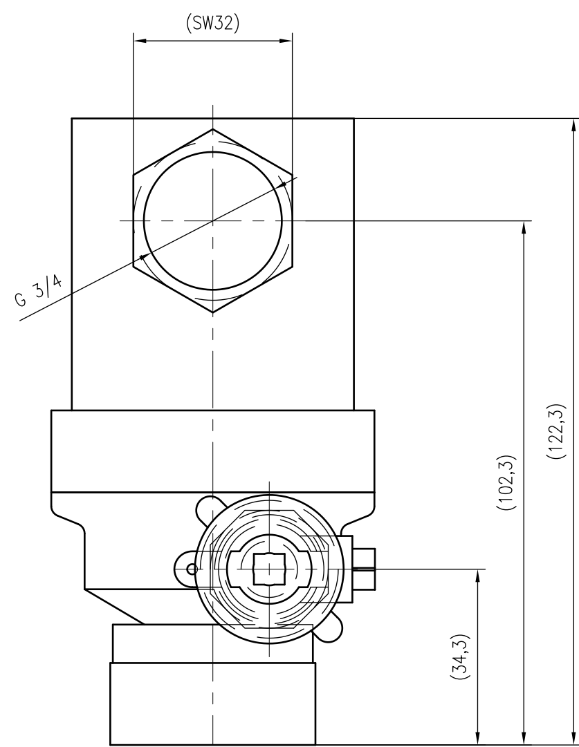
Side view
