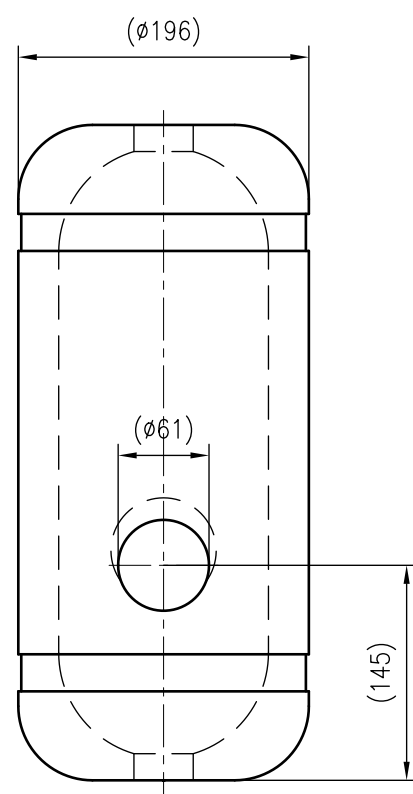
Side view
