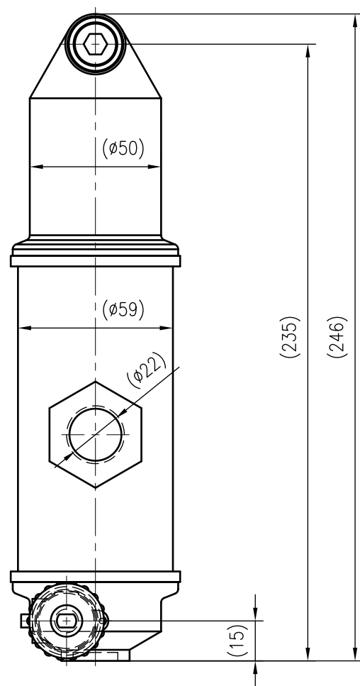
Side view
