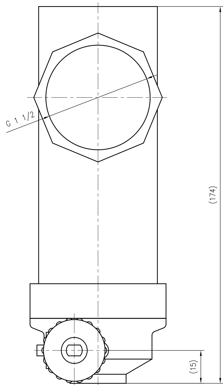
Side view
