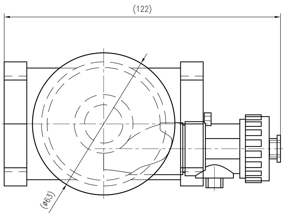
Top view
