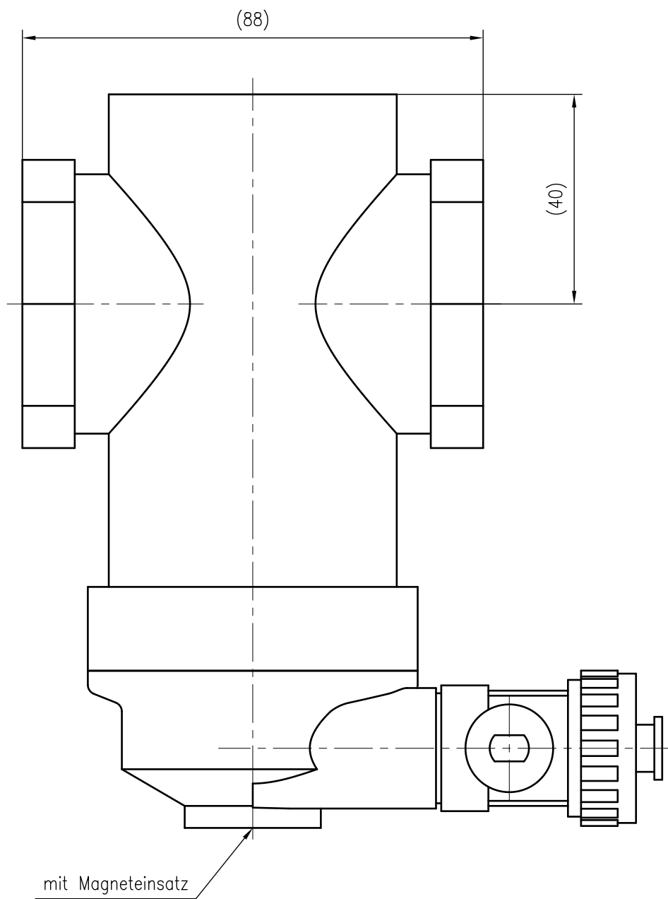
Front view
