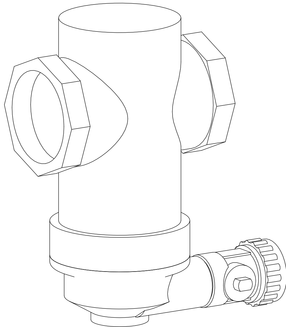
Isometric view
