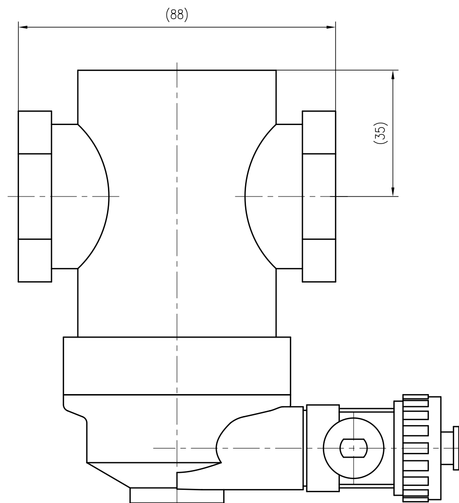
Front view
