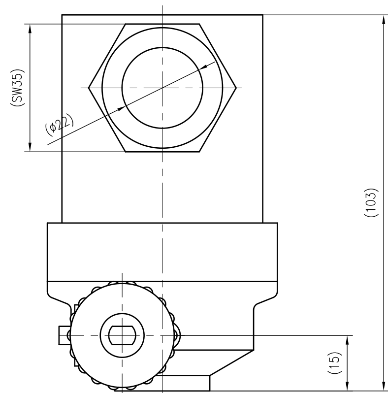
Side view
