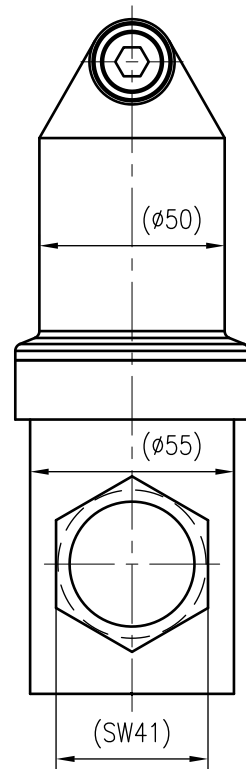
Side view
