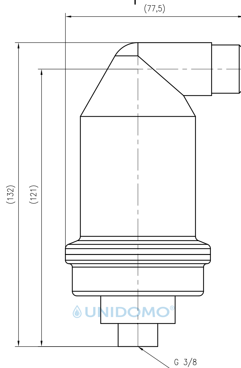
Front view
