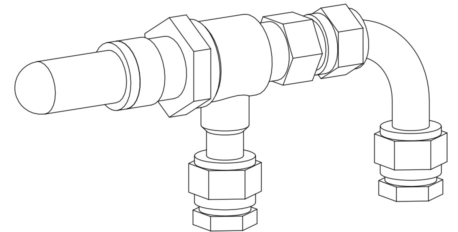
Isometric view
