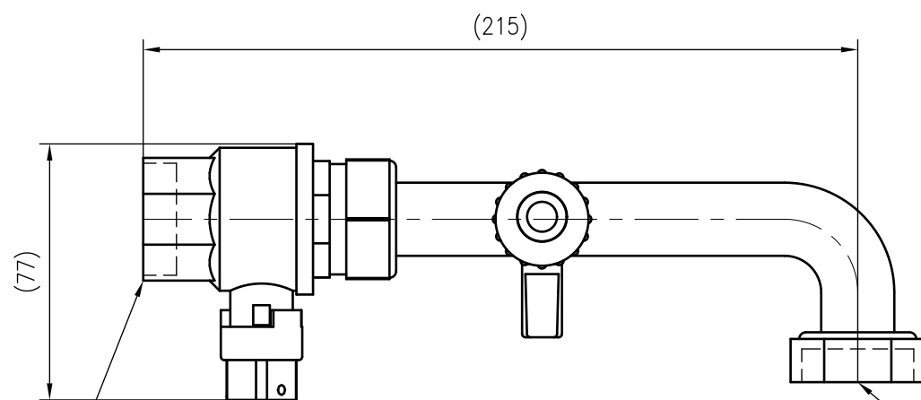
Top view
