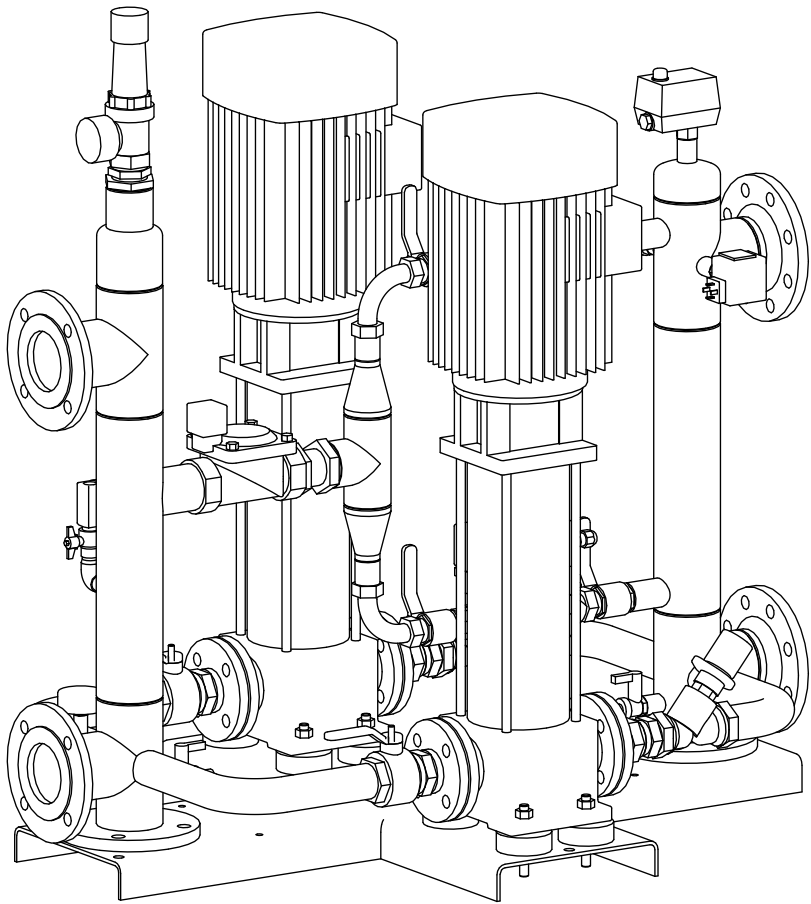
Isometric view
