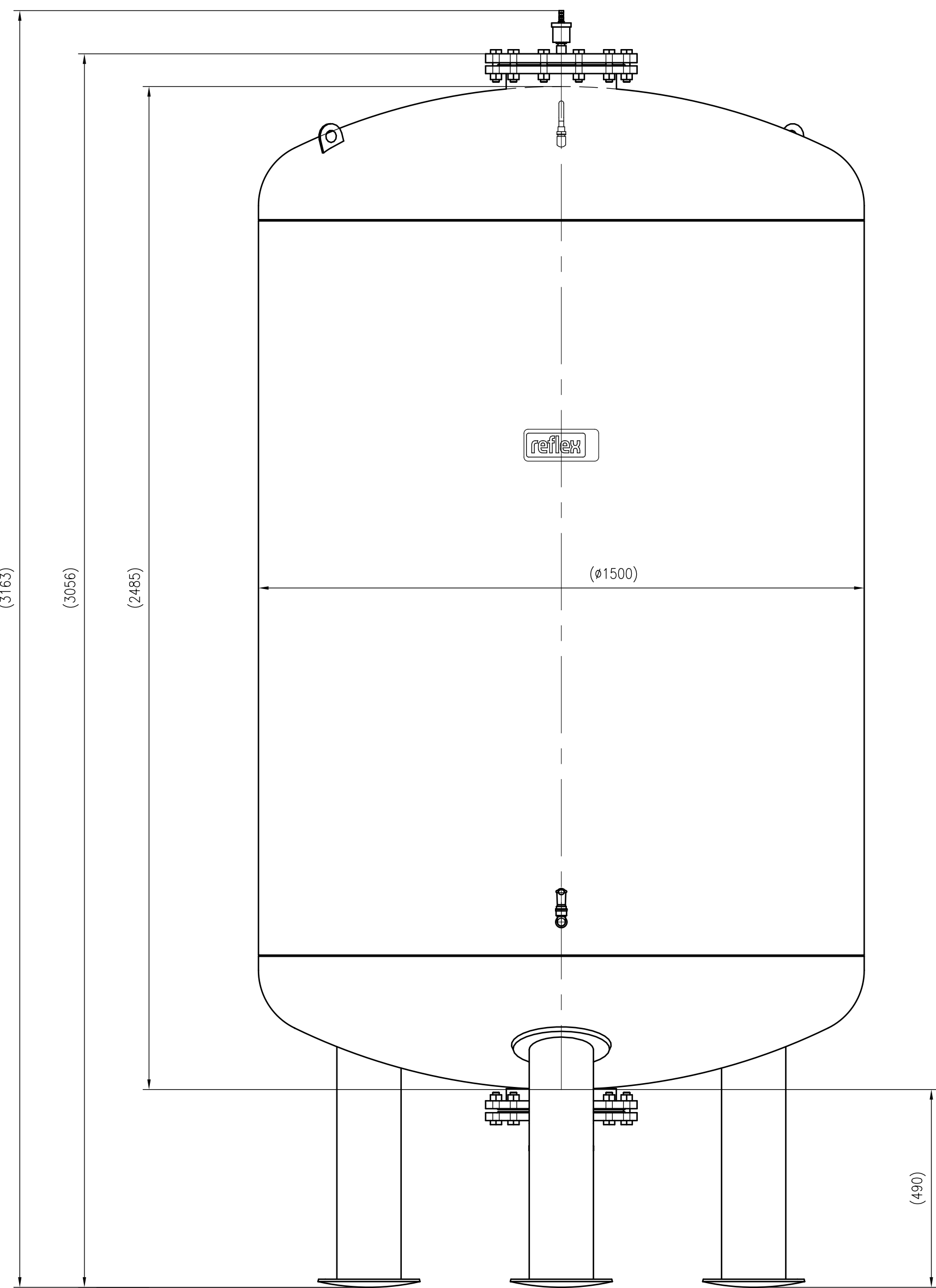
Front view
