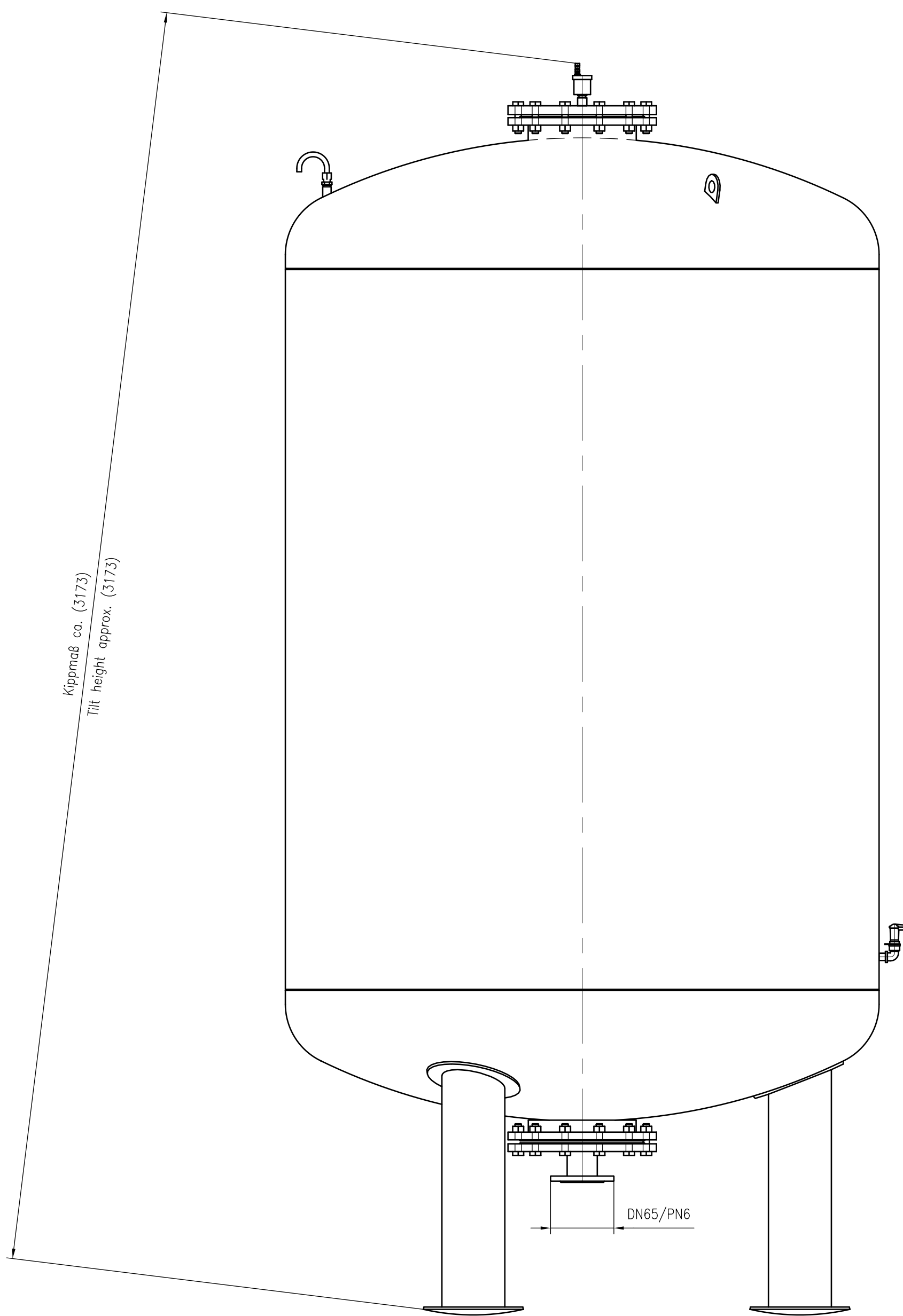
Side view
