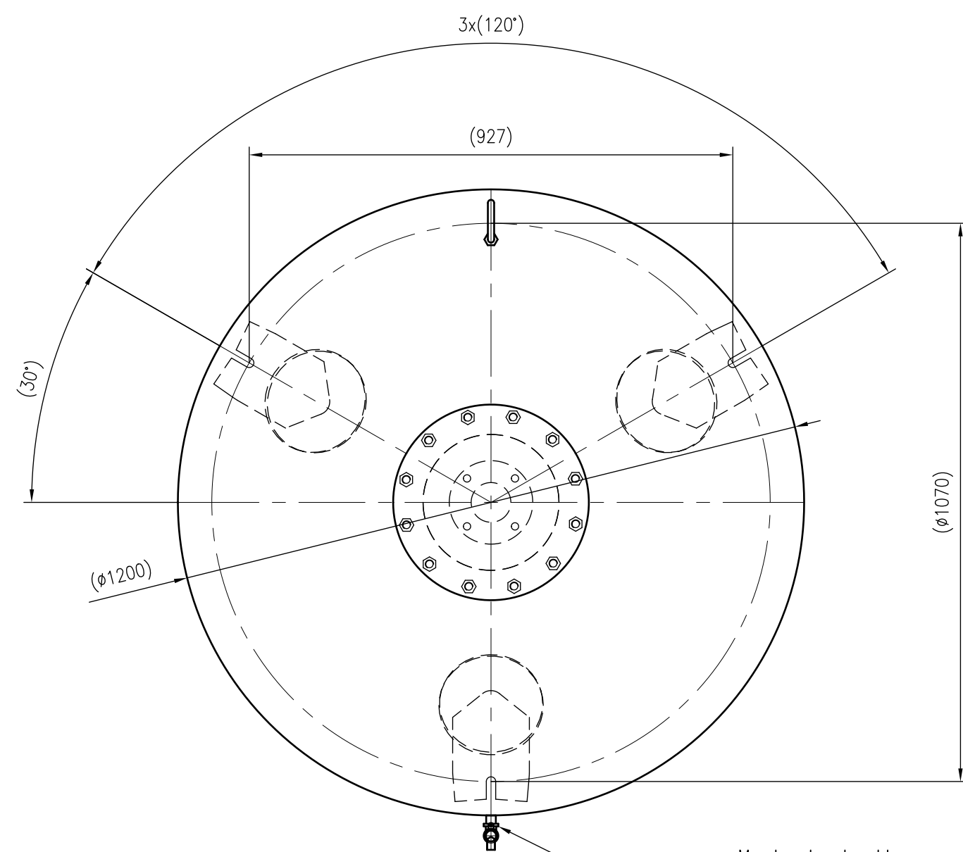
Top view
