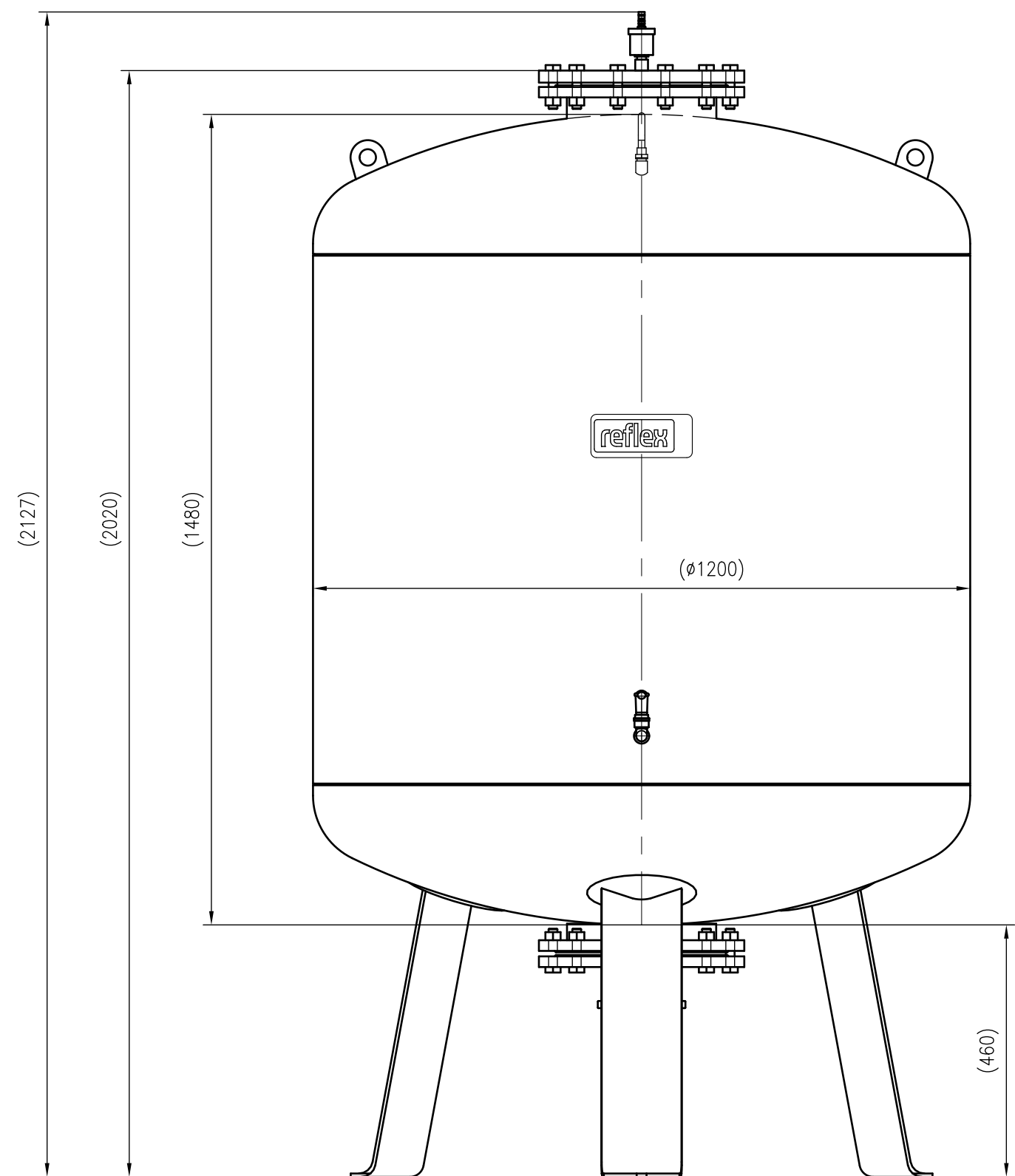
Front view
