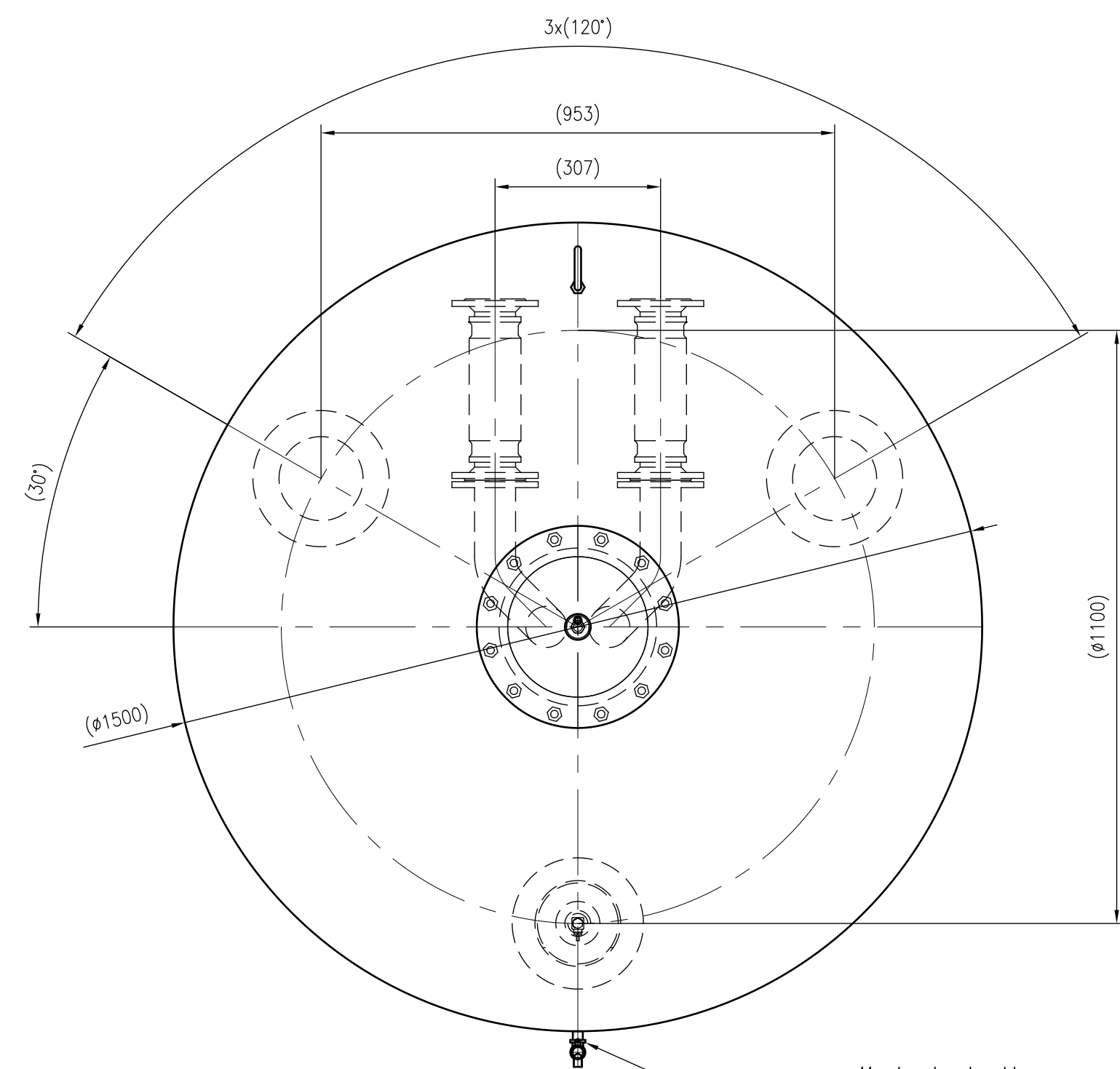
Top view
