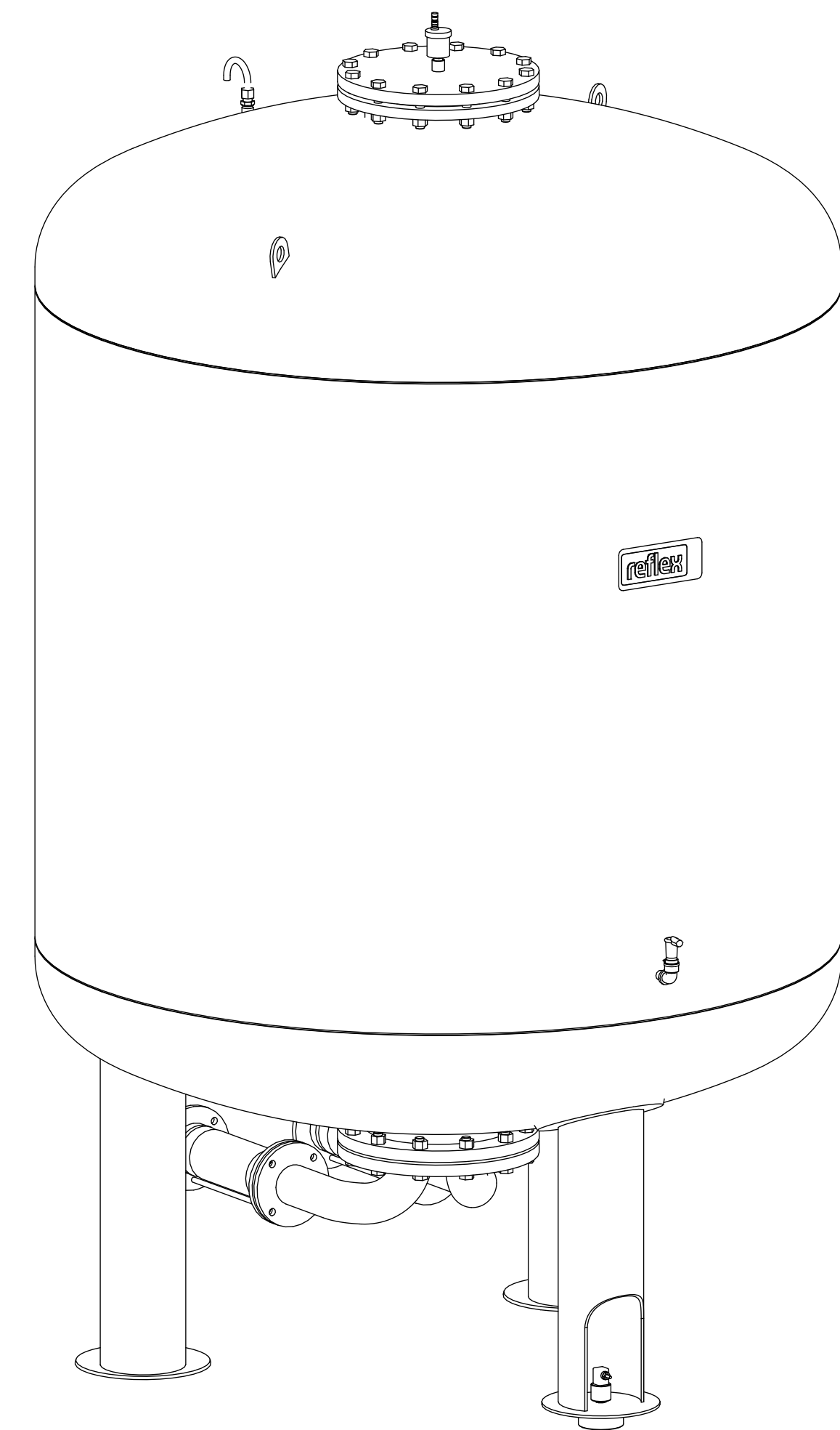
Isometric view
