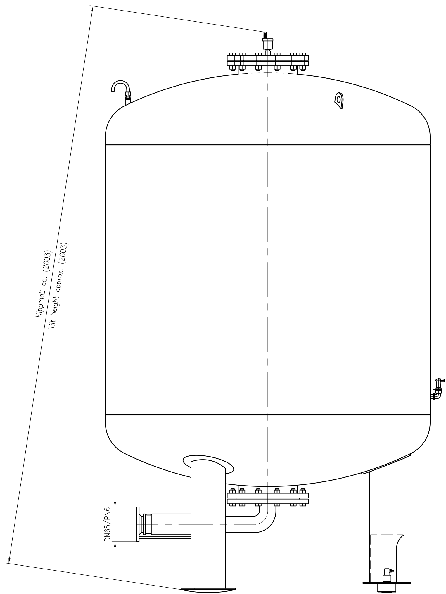
Side view
