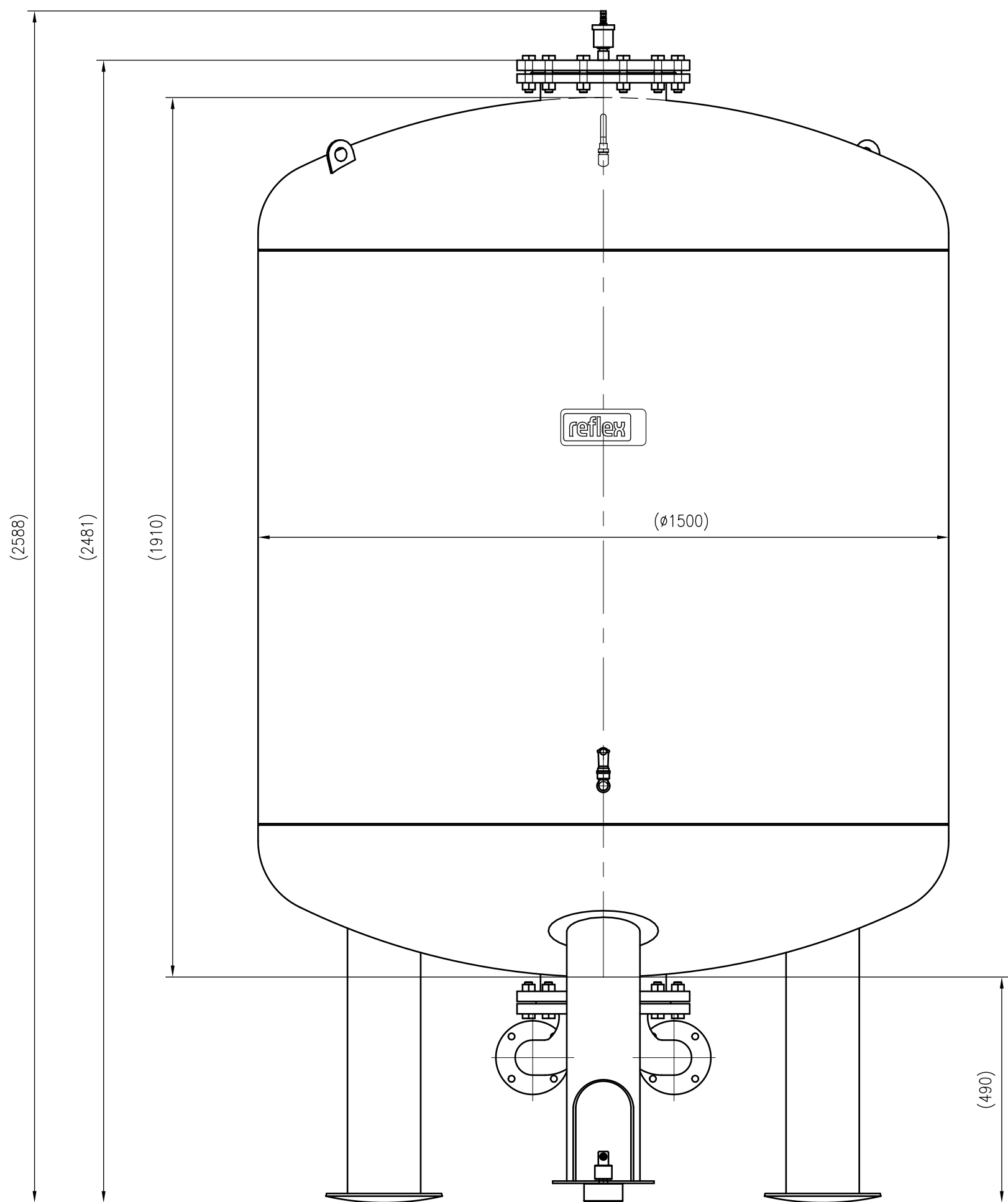
Front view
