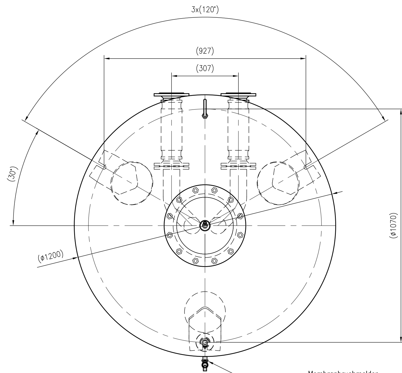
Top view
