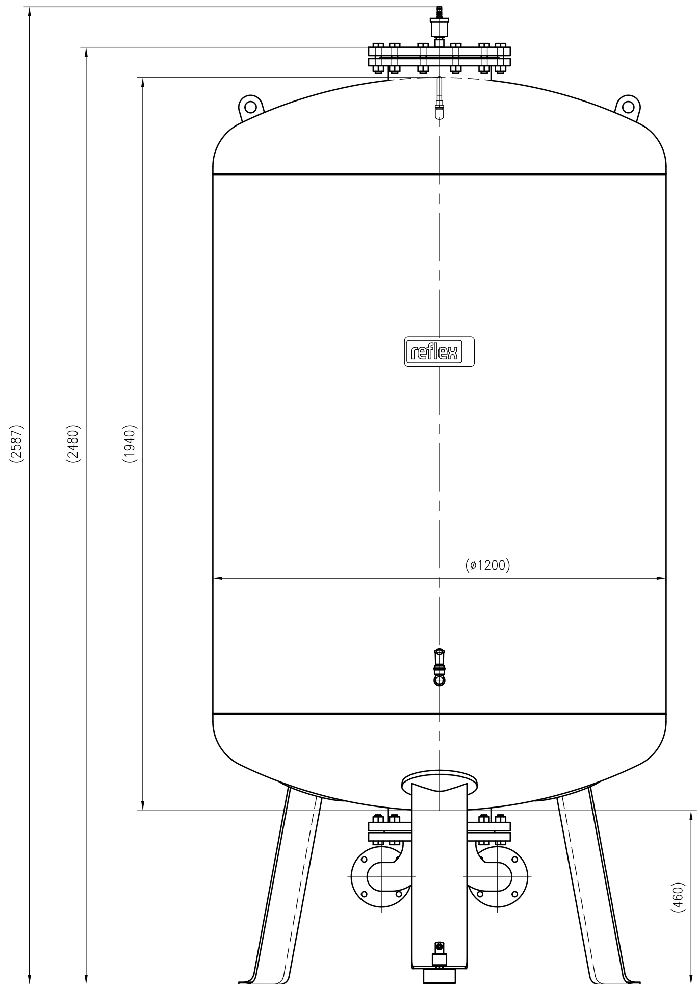
Front view
