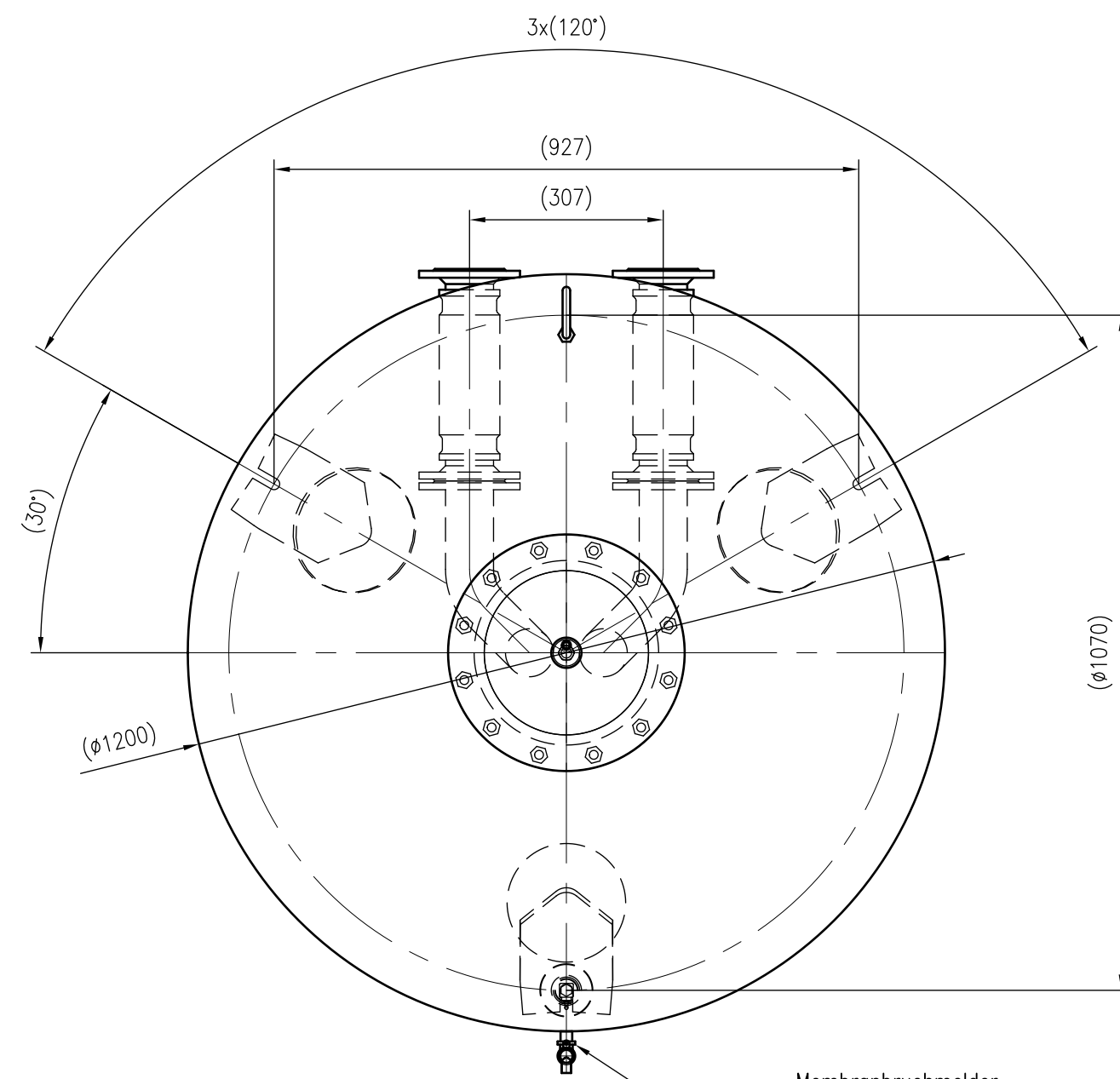
Top view
