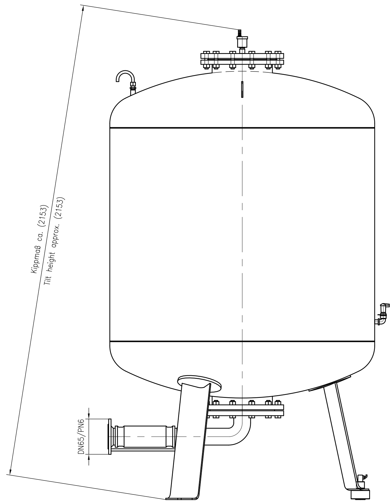
Side view
