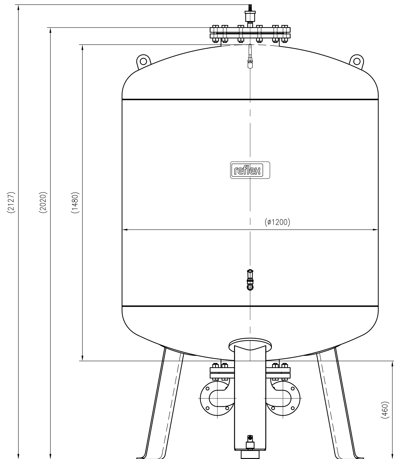
Front view
