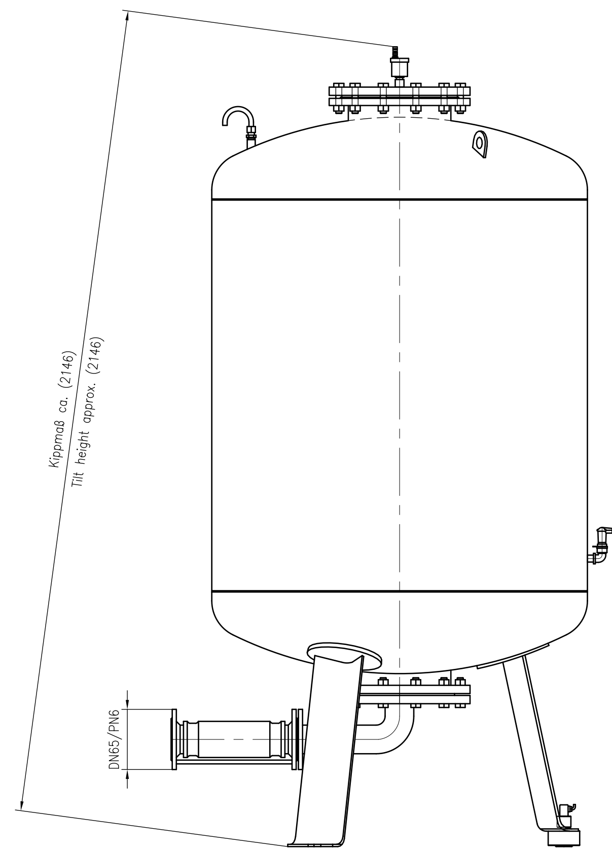
Side view
