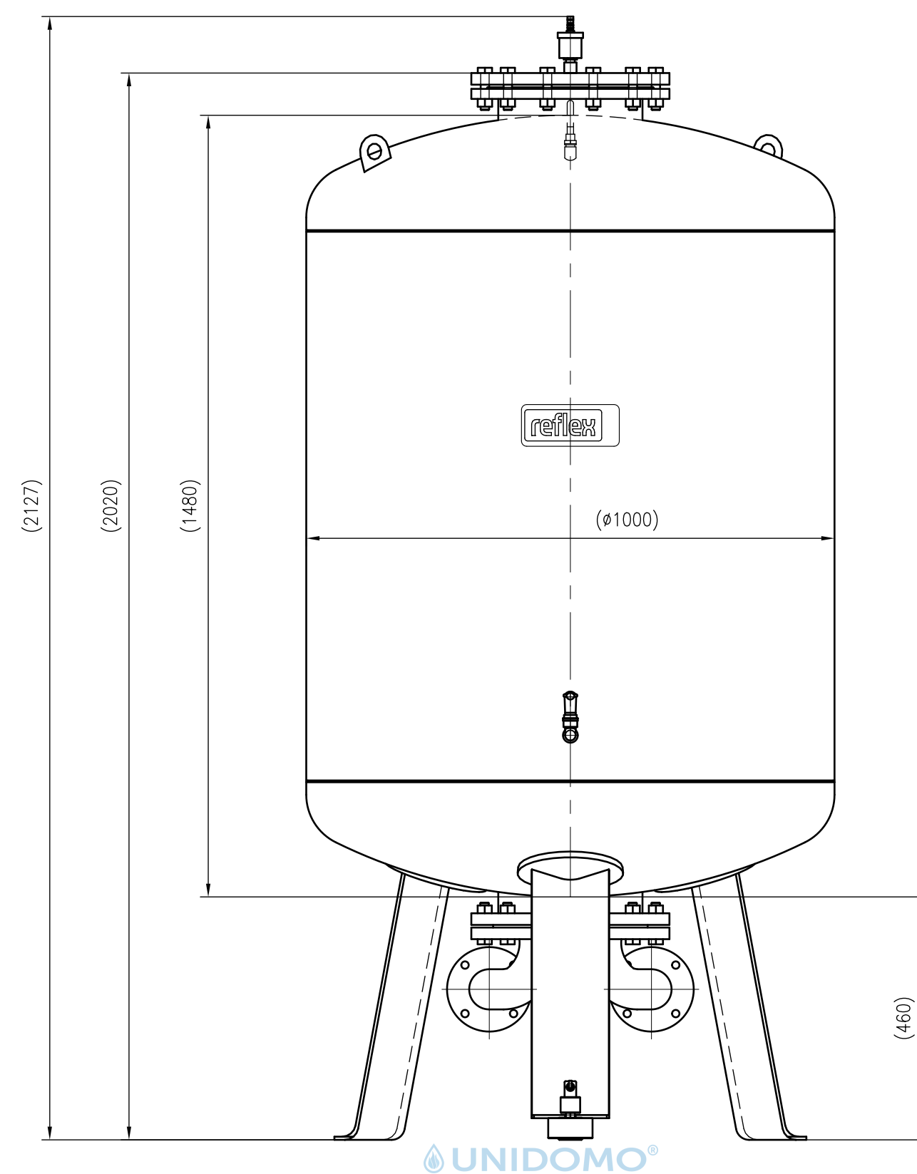
Front view
