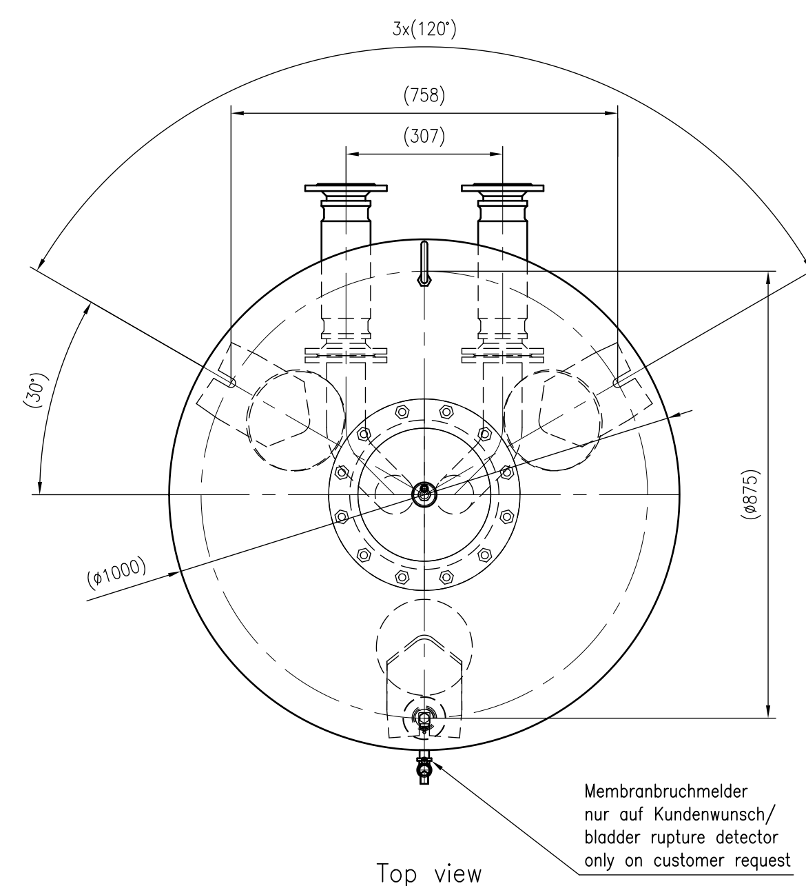
Top view
