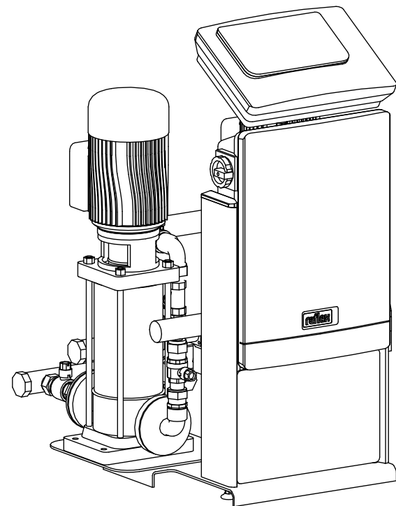
Isometric view
