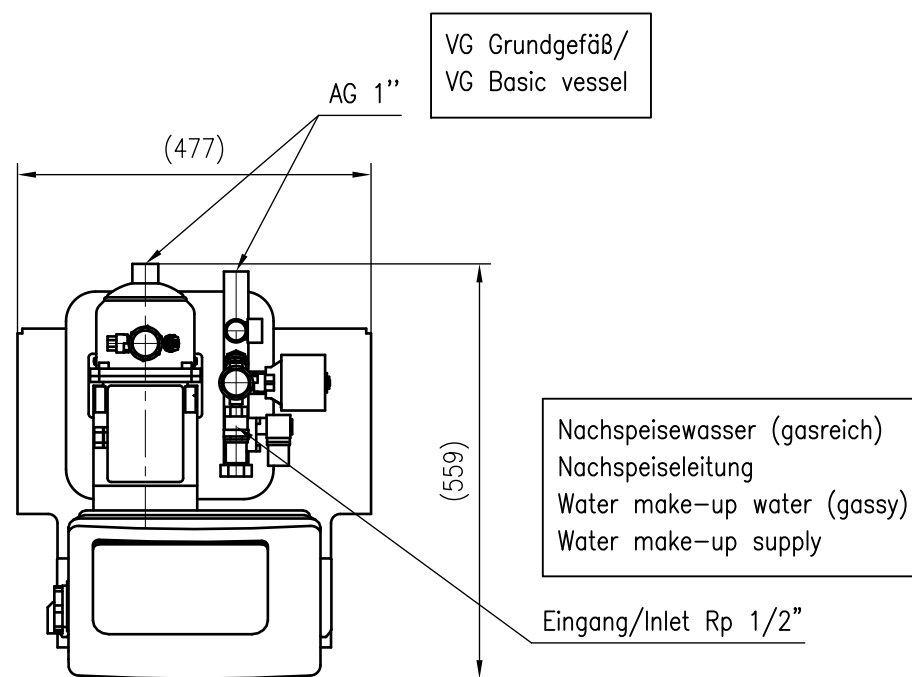
Top view
