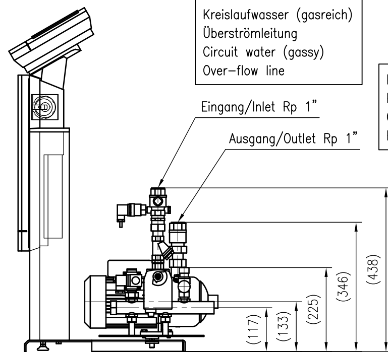
Side view
