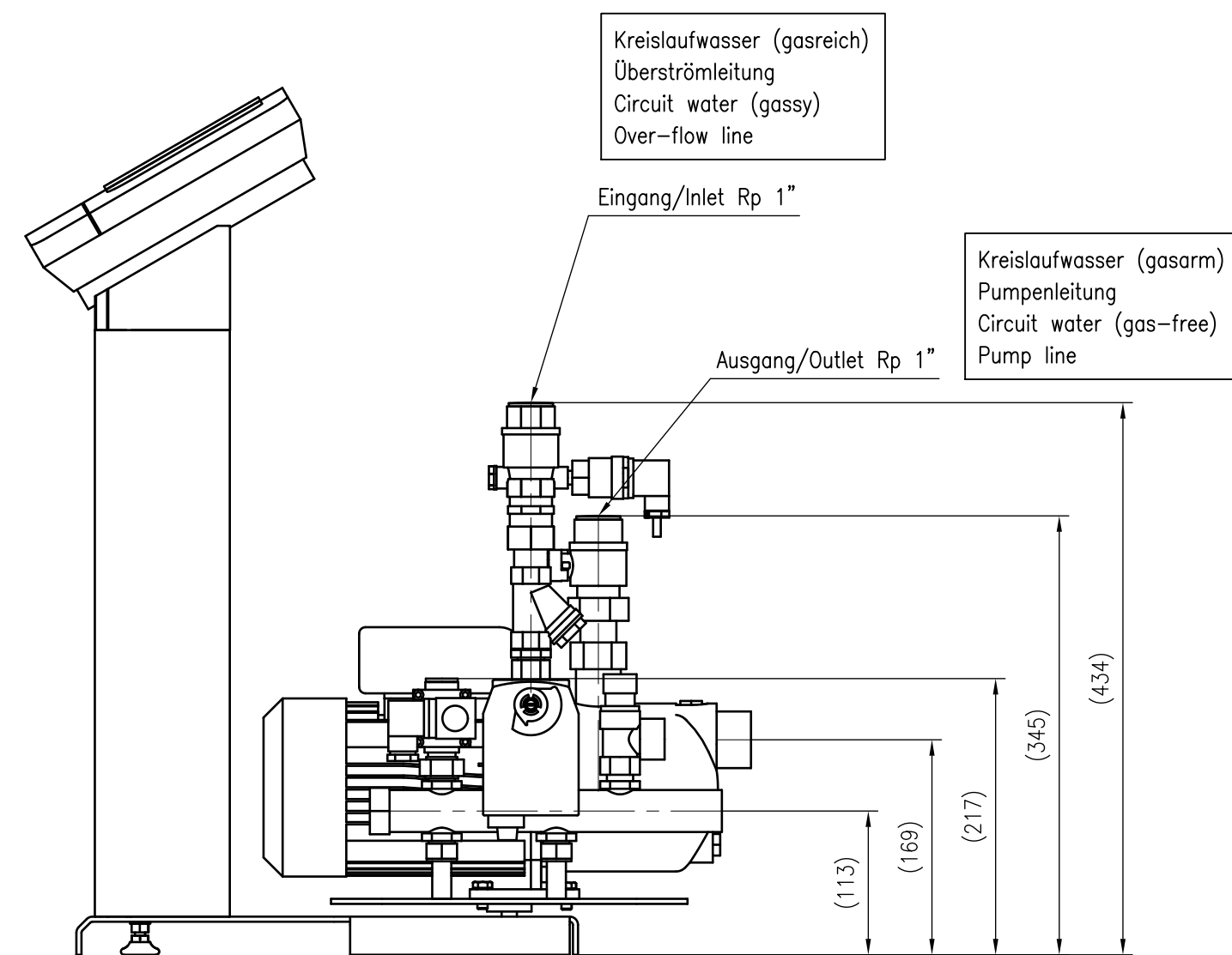
Side view
