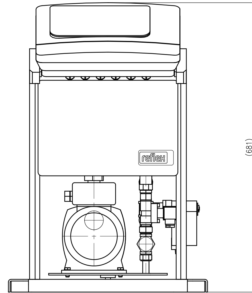
Front view
